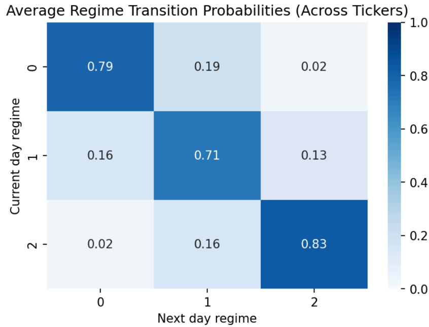
(Figure 5: Regime Transition Heatmap)
