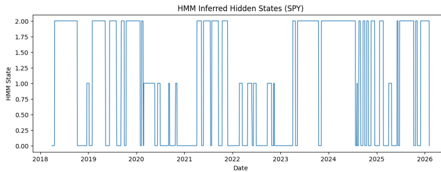
(Figure 6: HMM States Over Time)
