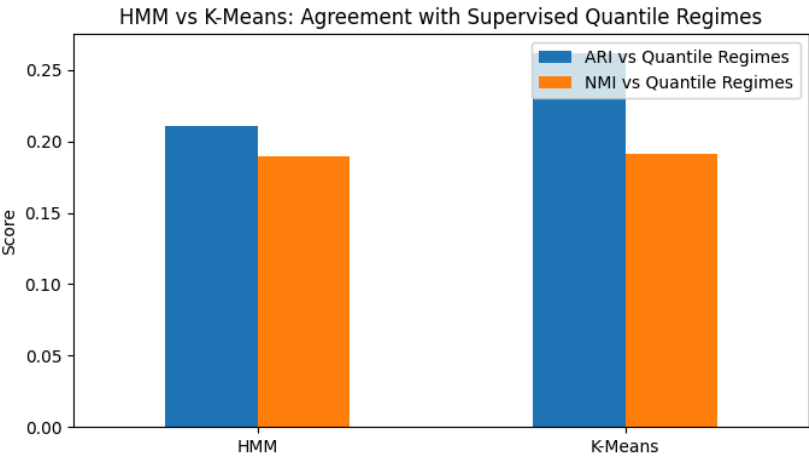
(Figure 11: ARI/NMI Comparison — HMM vs K-Means vs Quantile Regimes)
